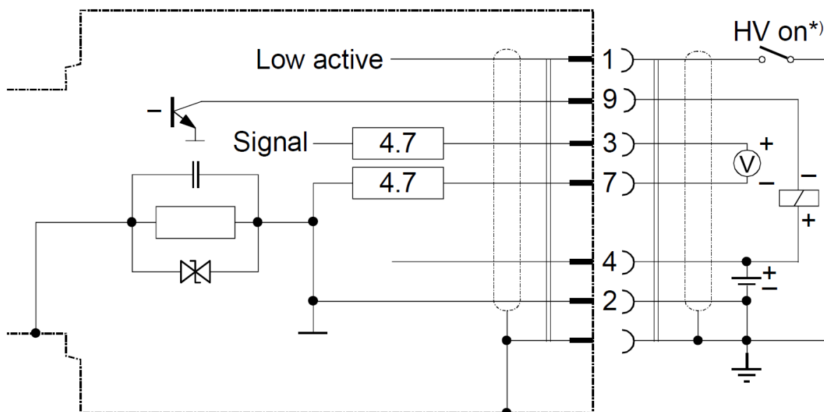
Wiring Diagram
